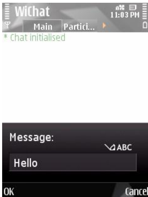
Figure 1. Message query
