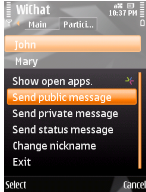
Figure 4. Options menu
